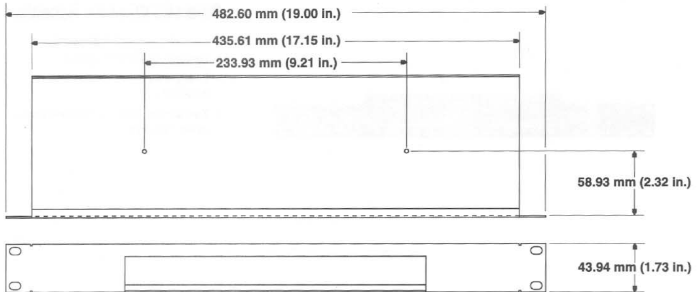
FIGURE 1 — Dimensions
